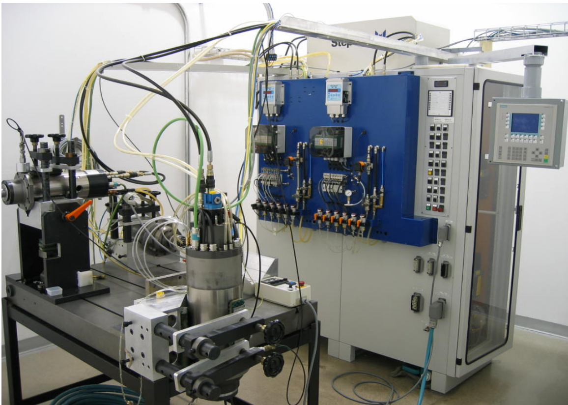
Test cell, equipped with two Siemens Universal Drives, 200 & 300 Ampere Drives, full periphery equipment to test all options on the Step Tec Spindles. Monitored via an 8 Channel Data Logger and a Simatic C7 Controller
